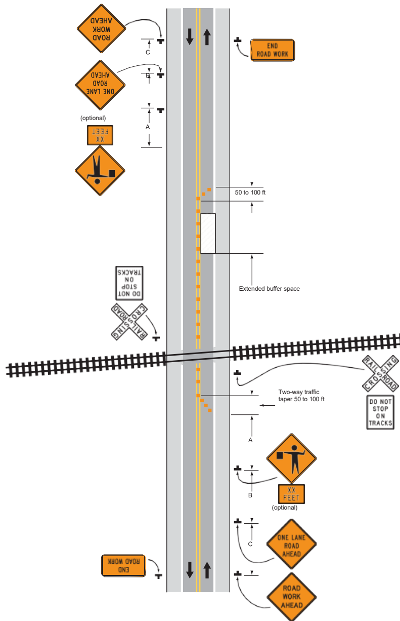
Work in the vicinity of a grade crossing
