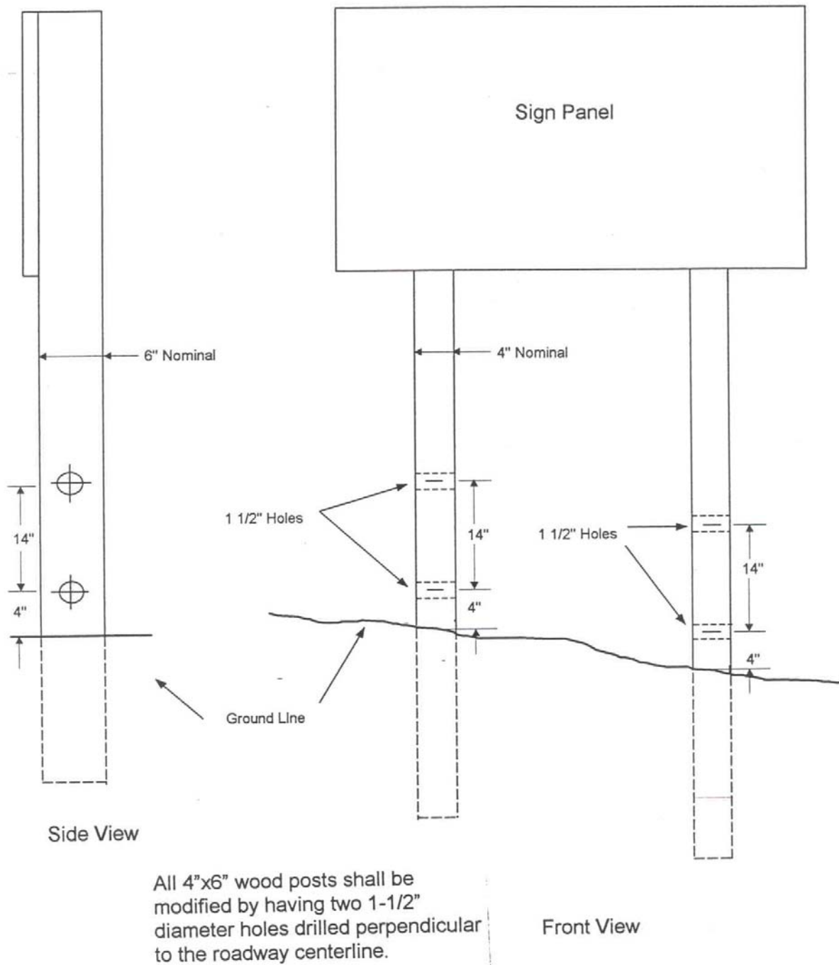
Typical Modification for Wood 4"x6" Sign Posts
